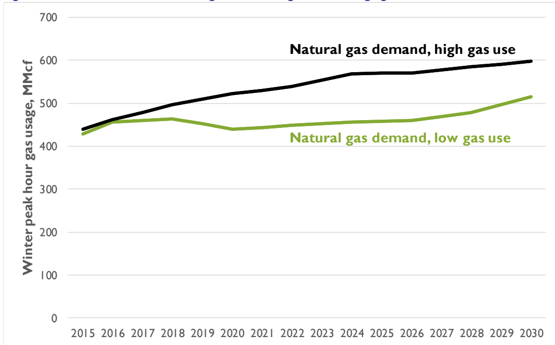
Figure ES-1. Peak demand for natural gas in the low gas use and high gas use scenarios
